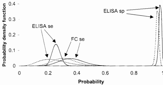
Figure 1. Probability distributions for ELISA sensitivity ( se ) and specificity ( sp ) and fecal culture ( FC ) sensitivity for the Mycobacterium avium paratuberculosis risk introduction model based on opinions of 2 subject matter experts (expert 1, solid lines; expert 2, dashed lines). (Specificity of FC was not fixed exactly at 100% [not shown] because of the possibility that M. a. paratuberculosis might be transiently present in feces without concurrent infection. 23 However, the likelihood of this phenomenon was considered to be low, and the expert estimations of FC specificity were >0.995 with a probability of at least 99%.)
